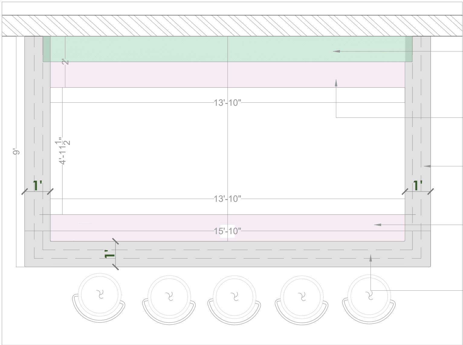
BAR COUNTER PLAN
